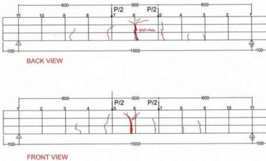
Figure 6. Crack pattern occurred at beam strengthened with 2 layer of wire mesh (B2)
