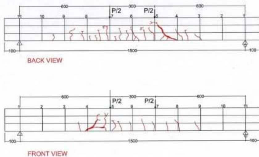
Figure 7. Crack pattern occurred at beam strengthened with 2 layer of wire mesh and 2 layer of GFRP (B3)
