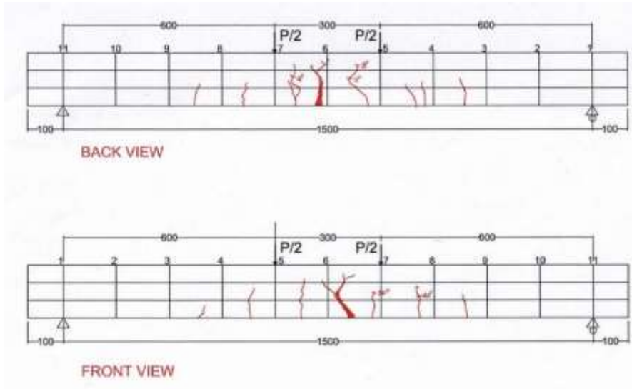
Figure 5. Crack pattern occurred at control beam (B1)
